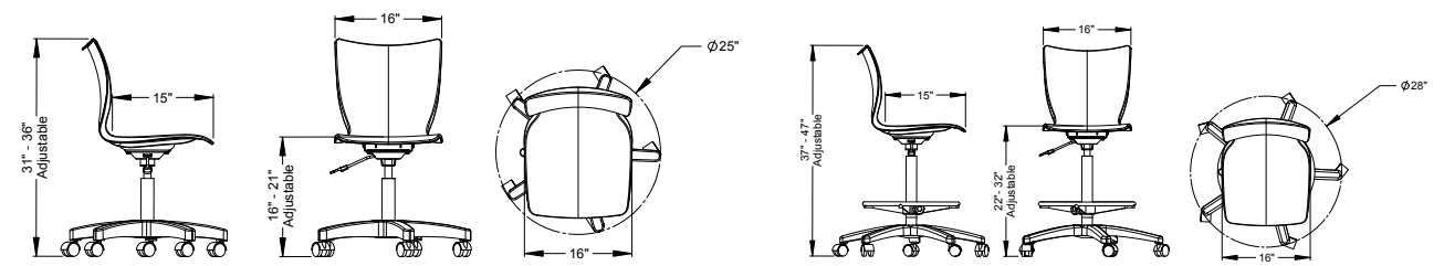
Adjustable Chair (A-Shell)
