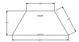
35" Deep Planner Work Center Top View
